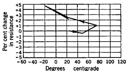
FIG. 2-10.—Changes of an unconditioned resistor with temperature.
