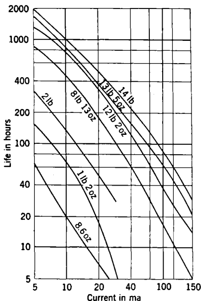
FIG. 12-1.—Battery life vs. current.
