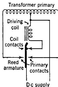
FIG. 12-22.—Series-drive vibrator circuit.
