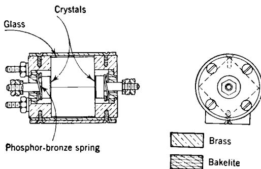
FIG. 7-24.—Glass 6- \mu sec delay line.
