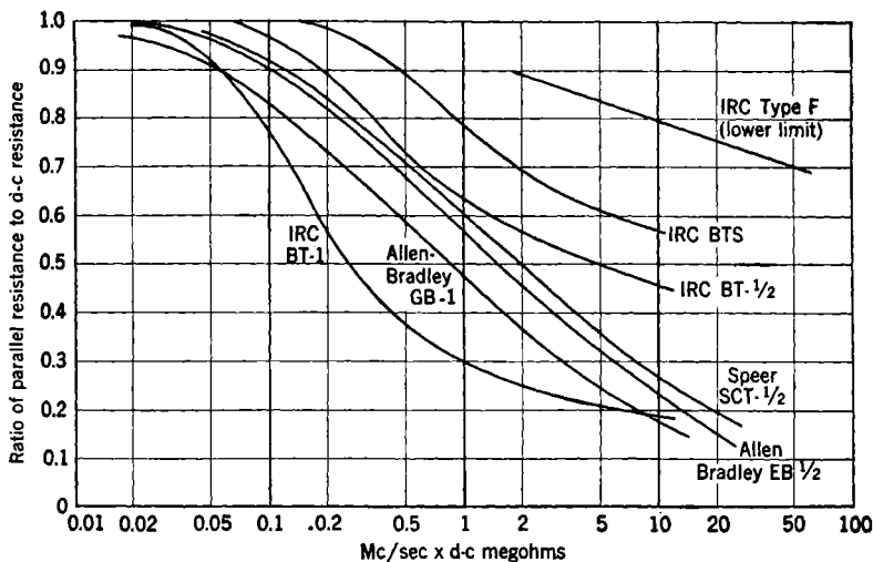
FIG. 2-21.—Resistance-frequency characteristics (1).
