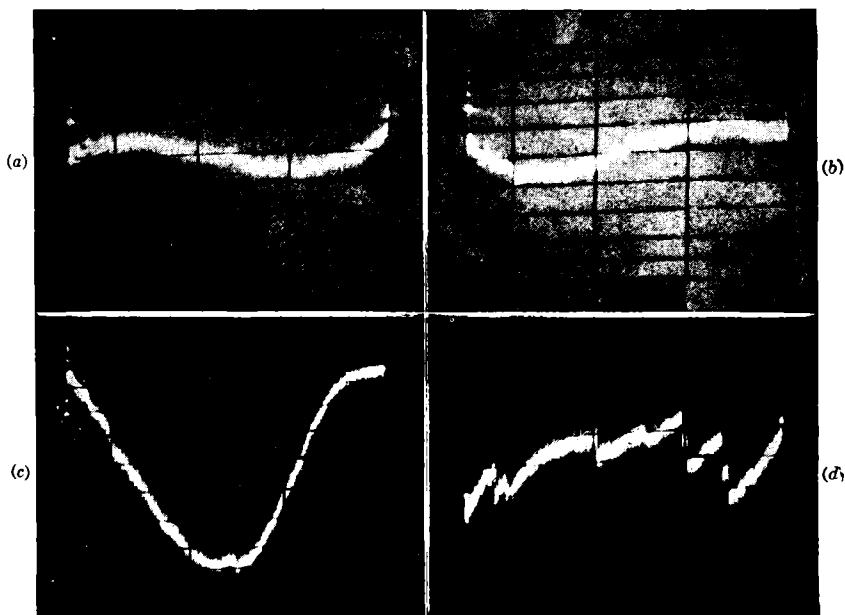
FIG. 8-17.—Effects of incorrect assembly techniques.
