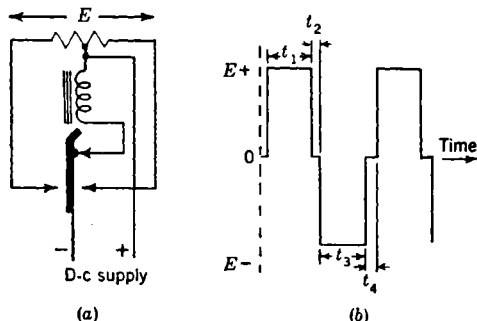
FIG. 12-23.—Vibrator with resistive load.
