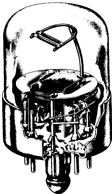
FIG. 14-11.—Twin high- \mu triode 7F8.
