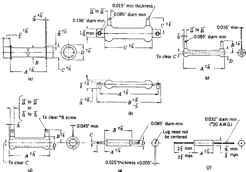
FIG. 3-2.—Power-type resistor dimensions.
