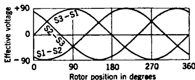
FIG. 10-4.—Navy synchro stator voltages.
