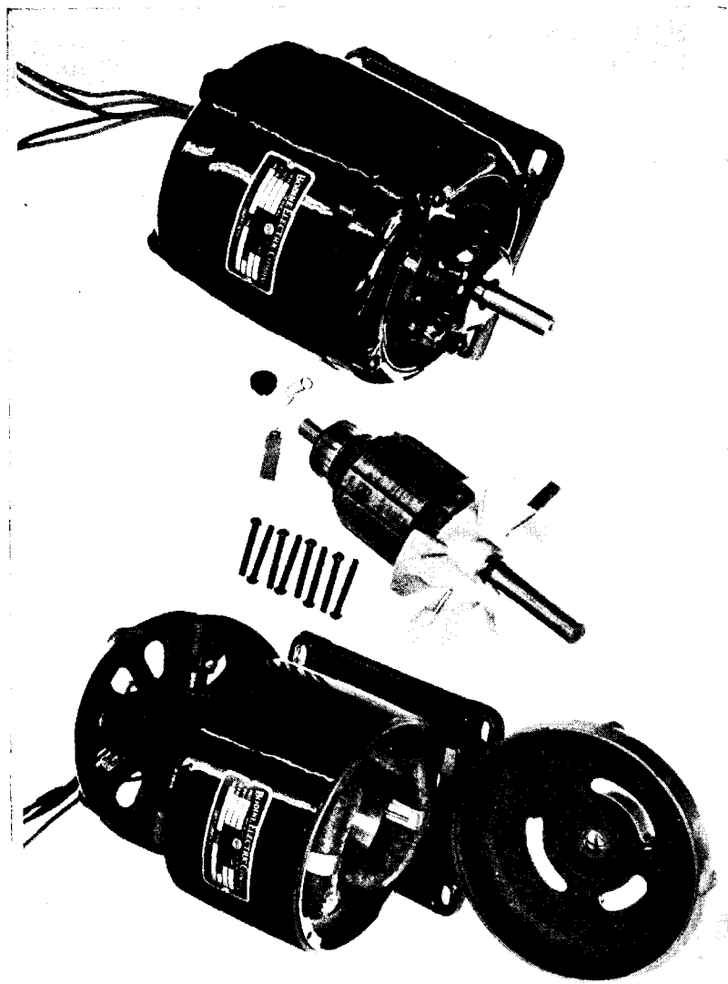
FIG. 11-1.—Bodine compound-wound d-c motor or generator: 115 volts d-c, \frac{1}{8} hp, 1725 rpm, sleeve bearings.
