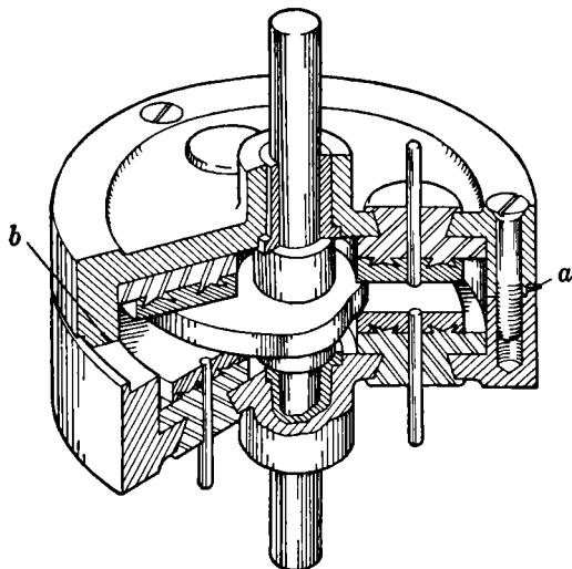
FIG. 9-10.—Nilsen condenser construction.
