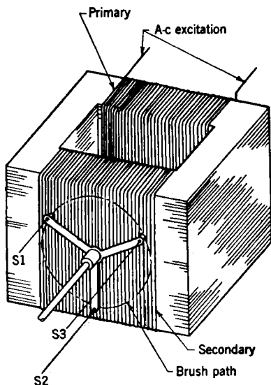
FIG. 10-10.—A-c commutator transmitter.
