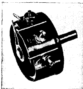
FIG. 8-26.—DeJur No. 12 potentiometer with Paliney contact.
