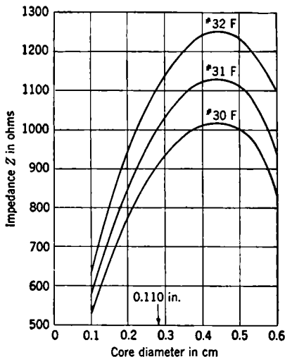
FIG. 1-9.—Cable impedance vs. core diameter.
