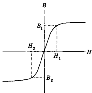
FIG. 10-31.—Magnetization curve of Magnesyn stator.
