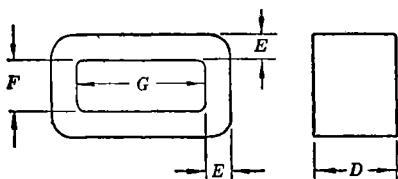
FIG. 4-21.—Radiation Laboratory standard Hipersil cores.
