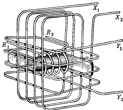
FIG. 10-38.—Telegon construction.
