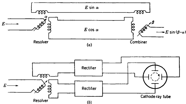
FIG. 10-26.—Use of 2-phase synchro as a resolver.
