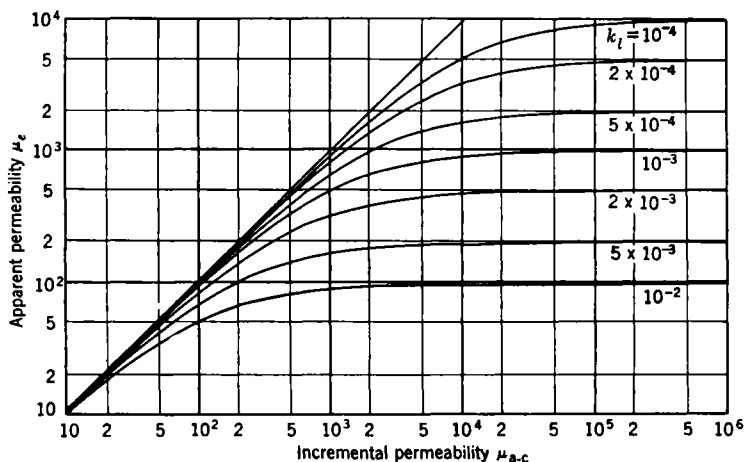
FIG. 4-5.—Effective permeability of core with air gap.
