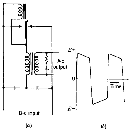
FIG. 12-25.—Series vibrator circuit.
