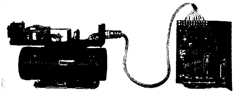
FIG. 12-35.—General Electric Company 150-volt aircraft inverter type PE-218-D, 115 volts, 400 cps, and electronic voltage regulator.
