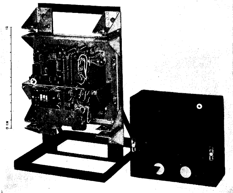
Fig. 12-34.—KS-15055 electronic voltage regulator designed by Bell Telephone Laboratories.
