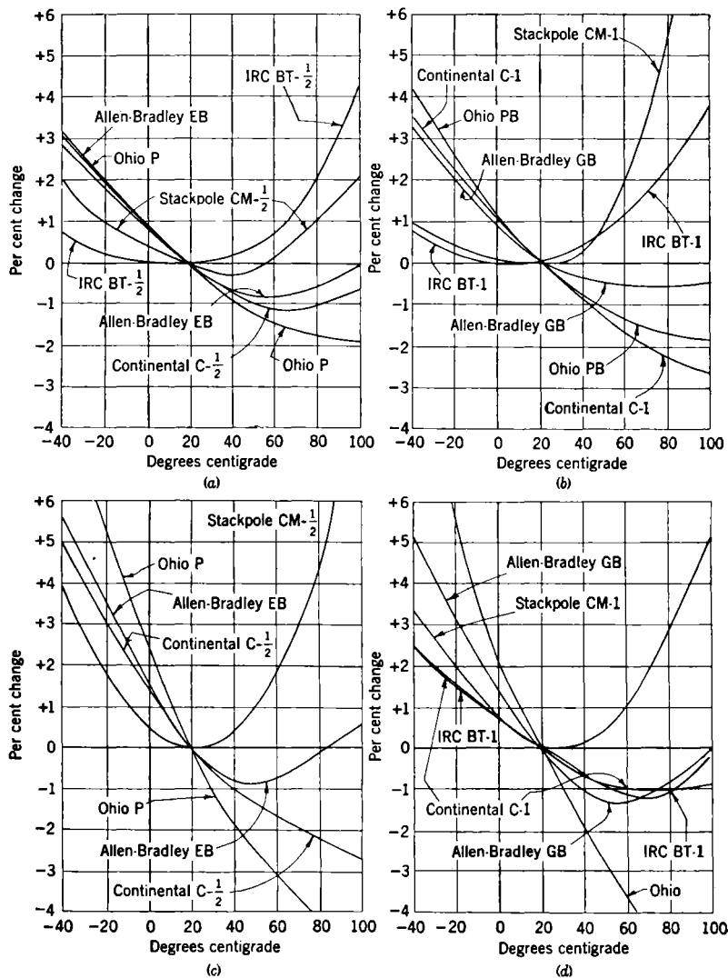
Fig. 2-11.—Resistance-temperature characteristics (1).
