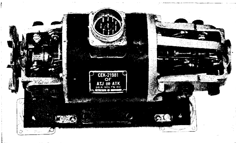
FIG. 12-5.—Eicor, Inc., aircraft dynamotor.
