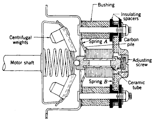
FIG. 12-16.—Holtzer-Cabot Electric Company carbon-pile speed governor.
