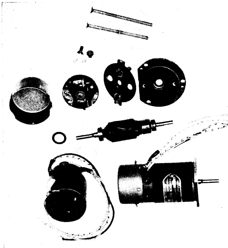
FIG. 11-22.—Delco constant-speed d-c series motor: 27-volt input, \frac{1}{10} hp, 6000 rpm, with Lee centrifugal governor; also made with adjustable-speed governor.
