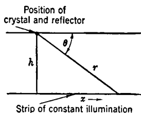
FIG. 5-11.—Geometry of reflector derivation.
