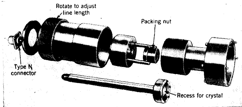
FIG. 7-17.—Variable end cell for Line D.
