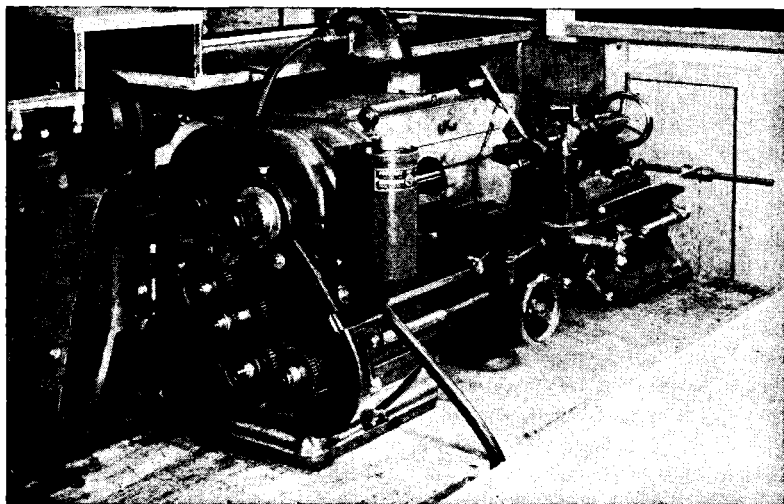
FIG. 8-8.—Round-mandrel winding lathe, side view.
