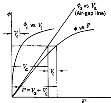
FIG. 4-6.—Sheared-curve construction. F = total magnetizing force. \phi = total flux. V_a = magnetic potential drop in air gap. V_i = magnetic potential drop in iron.
