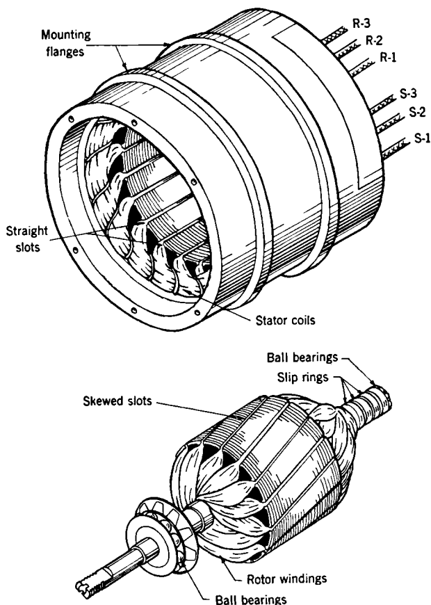
FIG. 10-7.—Synchro differential.
