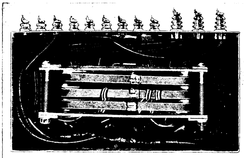
FIG. 4-14.—Three-phase transformer in case.
