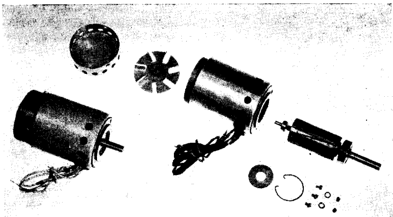
FIG. 11-9.—Eastern Air Devices variable-frequency capacitor-run a-c motor: with fan load, motor runs at nearly constant speed of 8000 rpm and output of \frac{1}{10} hp at all frequencies from 400 to 1800 cps; also made for single-frequency operation.
