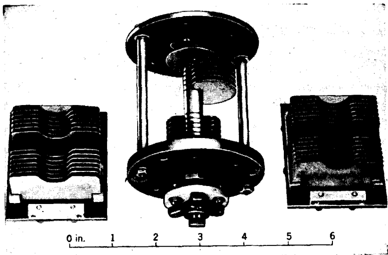
FIG. 9-3.—Cardwell condenser disassembled.
