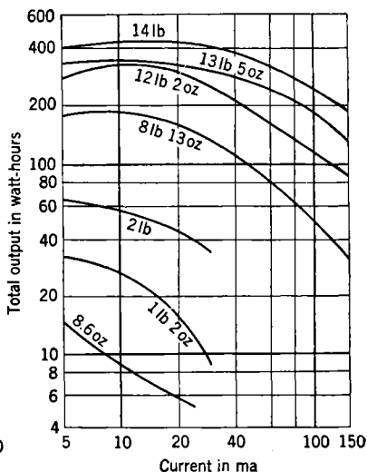
FIG. 12-2.—Total energy output vs. current.
