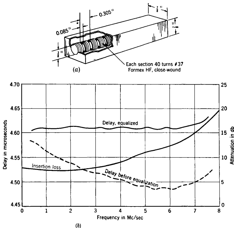
FIG. 6-22 (a and b).—BTL type D-172597 delay line.
