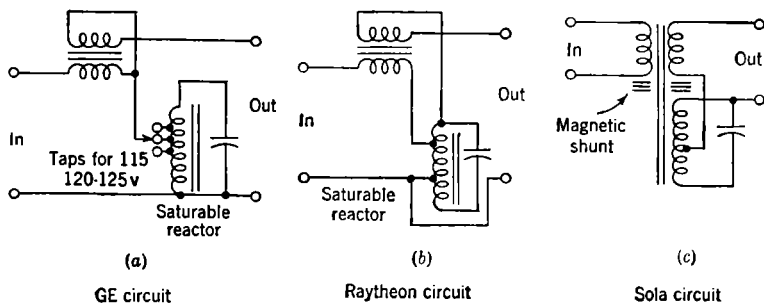
Fig. 12-38.—Commercial constant-voltage transformer circuits.
