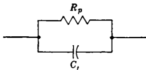
FIG. 2-14.—Simple equivalent circuit of a resistor.
