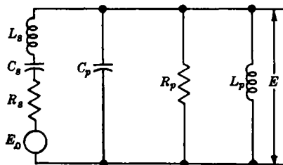
FIG. 5-7.—Equivalent circuit of crystal and tuning network.
