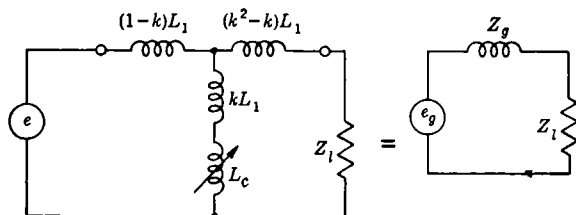
FIG. 12-44.—Equivalent circuit of electronic regulator.
