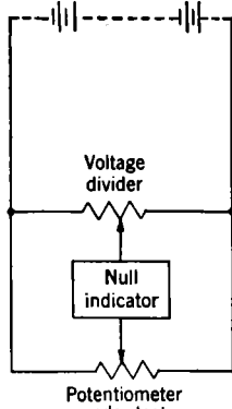
FIG. 8-19.—Basic circuit for ratio measurements.
