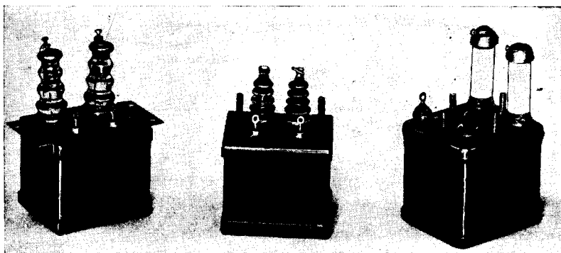
FIG. 4-17.—High-voltage transformers.
