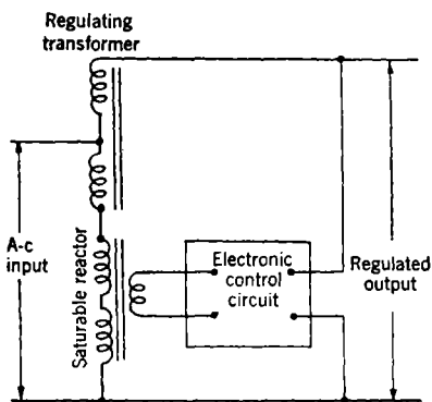
FIG. 12-41.—Basic circuit of electronic line-voltage regulator.
