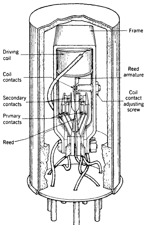
FIG. 12-19.—Typical low-power plug-in vibrator.
