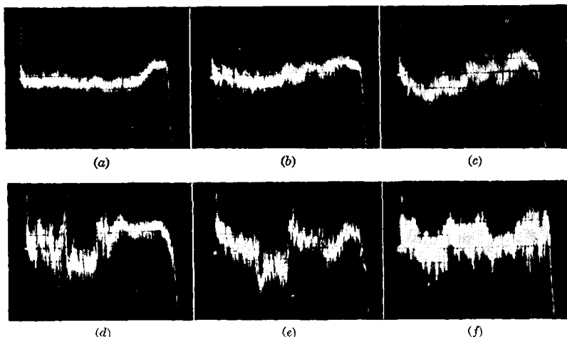
FIG. 8-10.—Linearity test of 3-in. 50,000-ohm potentiometer. (a) As delivered; brush pressure approximately 70 g; linearity 0.17 per cent; (b) taken at 10,000 cycles; linearity 0.22 per cent; (c) taken at 66,000 cycles; linearity 0.22 per cent; (d) taken at 202,000 cycles; linearity 0.32 per cent; (e) taken at 500,000 cycles; linearity 0.35 per cent; (f) taken at 1,002,800 cycles; linearity 0.28 per cent plus noise; brush pressure, 55 g, contact worn 0.0085 in. deep, area \frac{1}{4} by \frac{1}{8} in.
