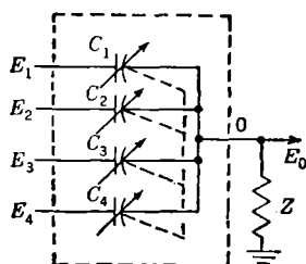
FIG. 9-1.—Schematic diagram of phase-shifting condenser.
