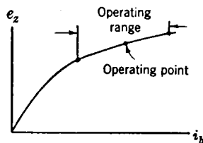
Fig. 12-37.—Voltage-current characteristic of saturable reactor.
