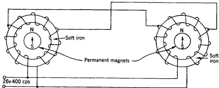
FIG. 10-35.—Rotary Magnesyne in back-to-back circuit.
