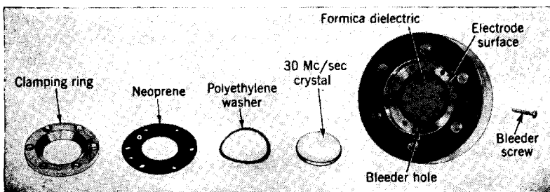
FIG. 7-9.—End assembly for Line C.
