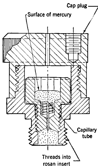
FIG. 7-4.—Mercury inlet with capillary loading.
