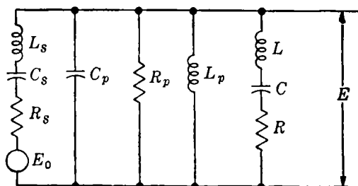
FIG. 5-9.—Crystal compensating circuit.
