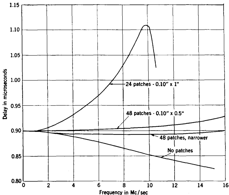
FIG. 6-9.—Effect of size and subdivision of patches.
