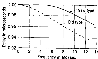
FIG. 6-13.—Effect of metal-paste dielectric.
