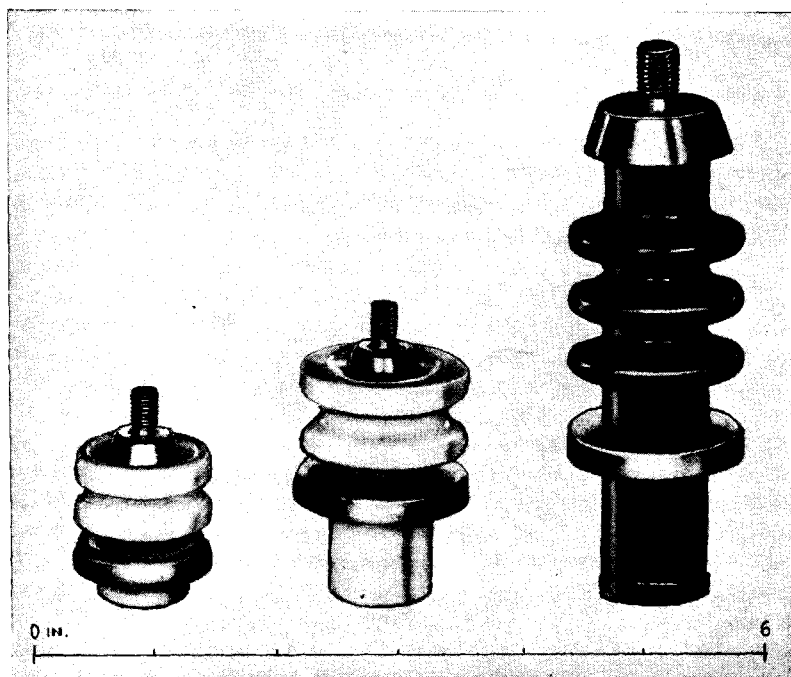
FIG. 4-31.—High-voltage bushings. (Left to right: C-12290-A; C-12966-A; C-13330-A.)
