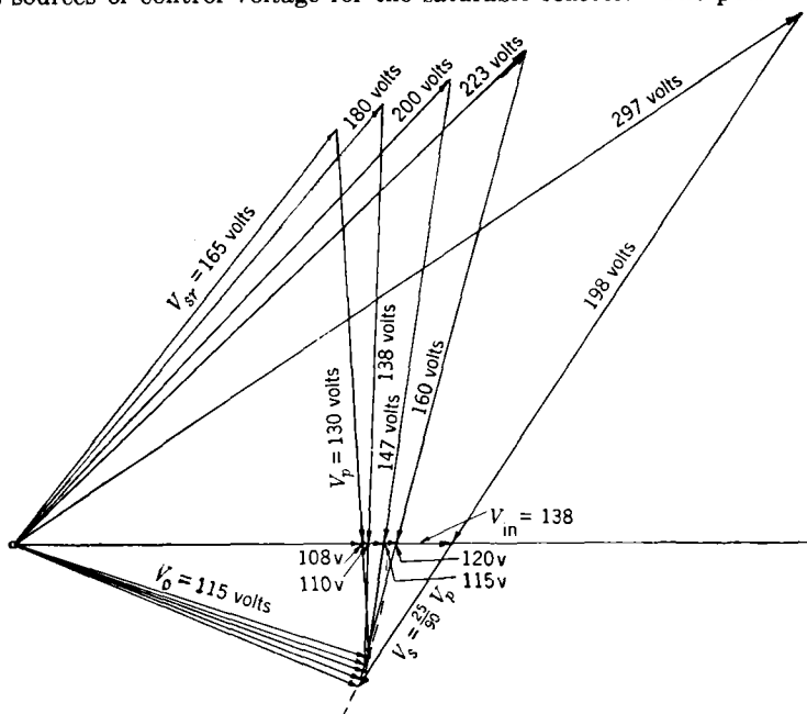
FIG. 12-42.—Fundamental vector diagram of electronic line-voltage regulator.
