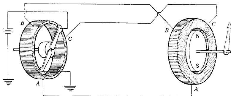
FIG. 10-43.—Three-wire three-coil d-c Selsyn system.
