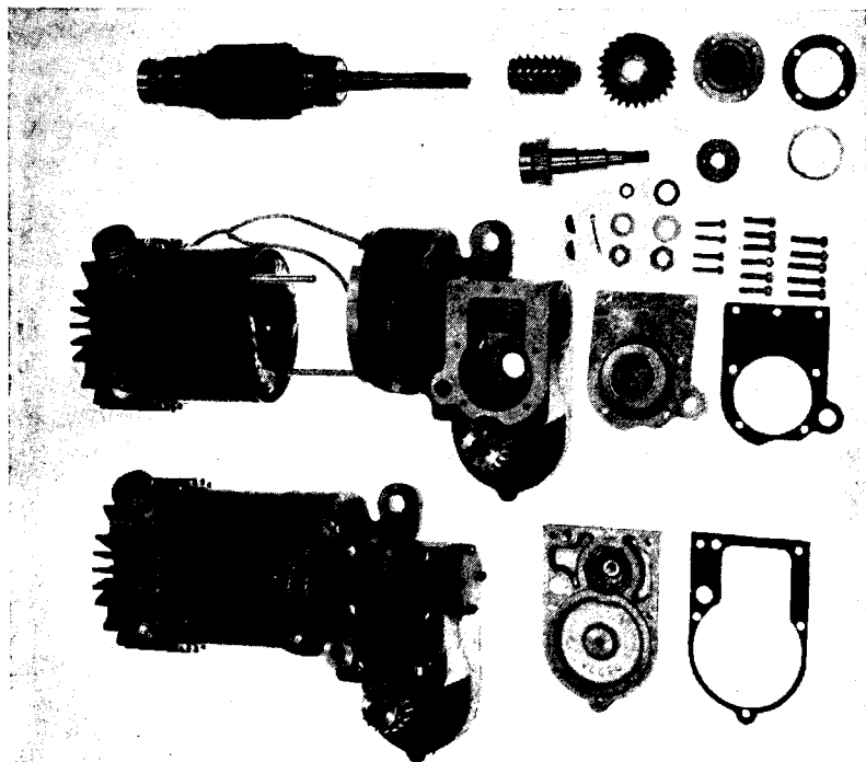
FIG. 11-19.—Oster double-commutator two-speed d-c shunt-wound motor: 27 volts, \frac{1}{2} hp; speed change obtained by series or parallel connection of the two armature windings.
