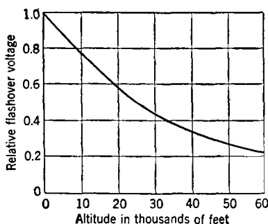
FIG. 4-32.—Derating curve for high-altitude operation.
