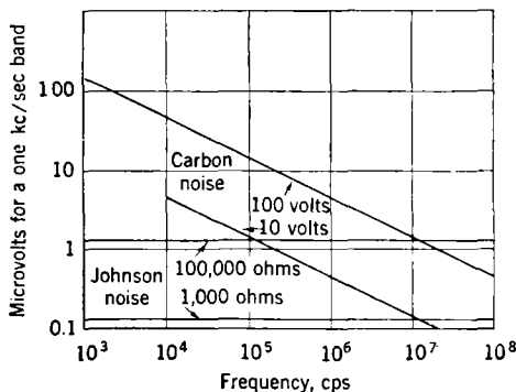
FIG. 2-13.—Resistor noise.
