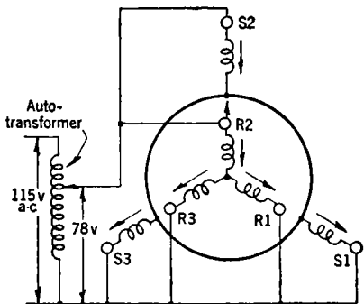
FIG. 10-21.—Zeroing a Navy synchro differential with rotor free to turn. When unit is connected as shown, rotor automatically assumes electrical zero position.
