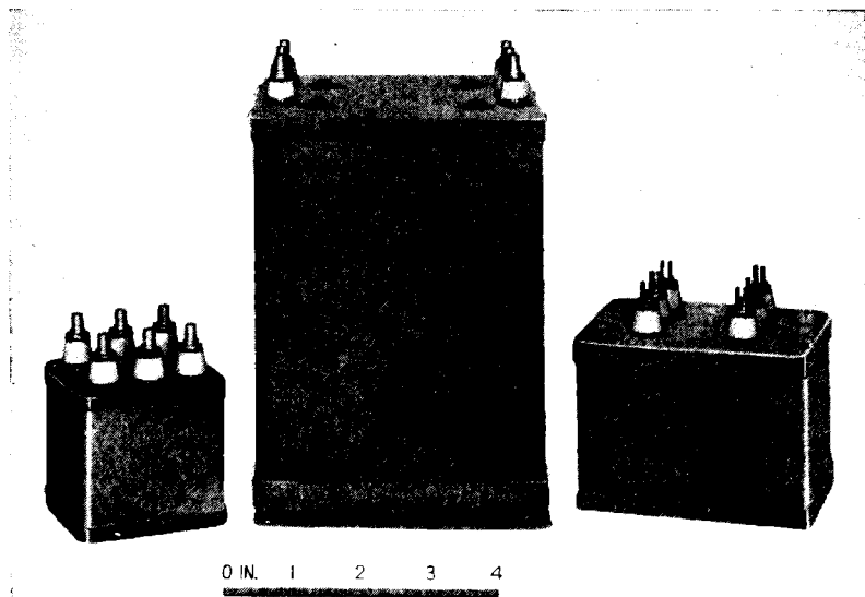
FIG. 10-25.—Synchro matching transformers.
