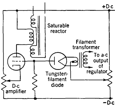
FIG. 12-43.—Emission-tube control circuit.
