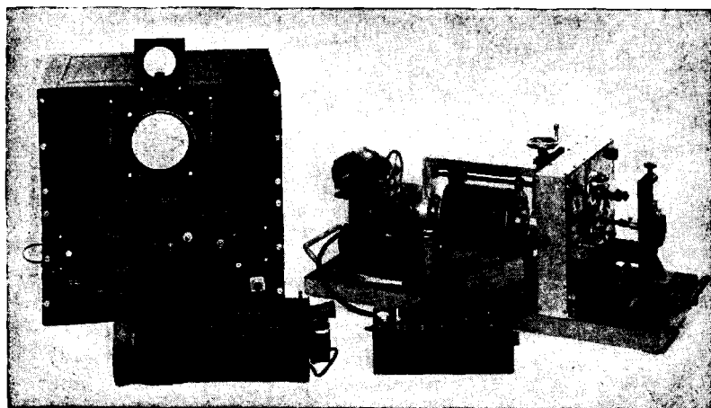
Fig. 8-21.—Continuous linearity testing assembly.
