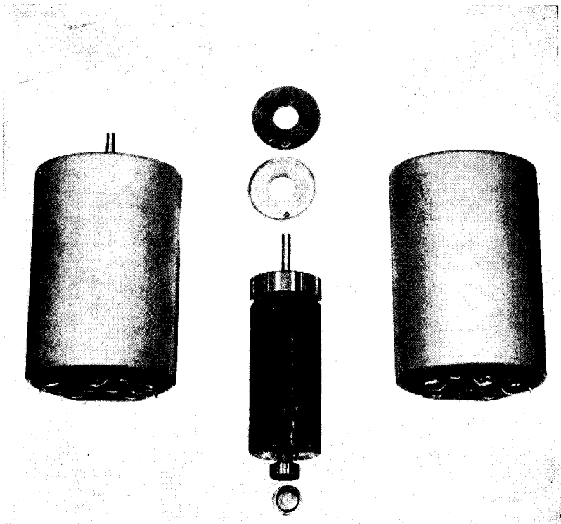
FIG. 11-10.—Eastern Air Devices 3-phase 400-cps synchronous motor: \frac{1}{10} hp, 115 volts, salient pole.
