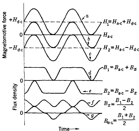
FIG. 10-32. —Magnetomotive force and flux in Magnesyn.
