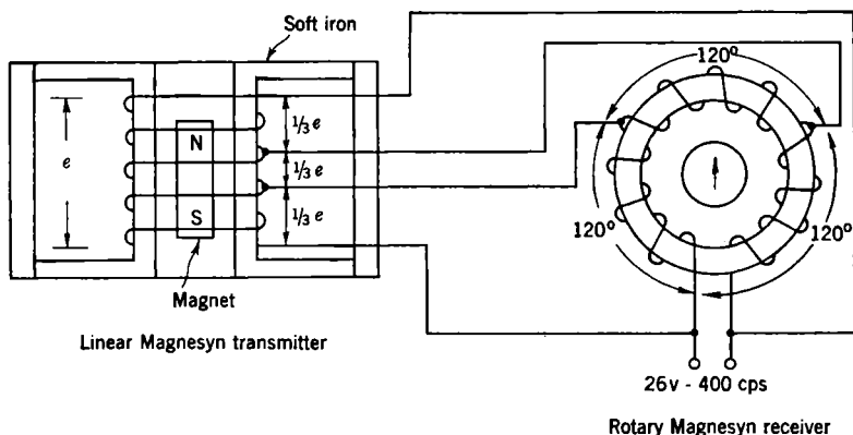
FIG. 10-36.—Linear and rotary Magnesyns back-to-back.
