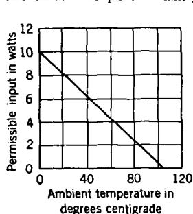
Fig. 8-18.—Power dissipation of type RL-270 potentiometer.
