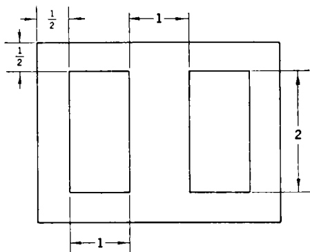
FIG. 4-22.—Most efficient lamination shape.
