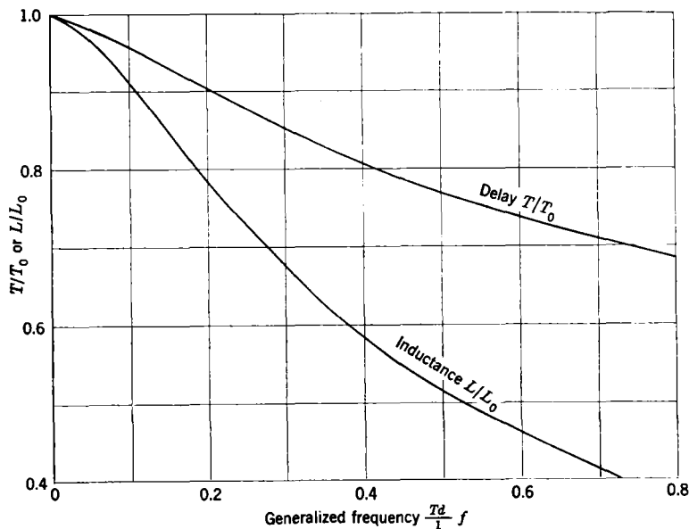
FIG. 6-1.—Effective inductance and time delay vs. frequency.
