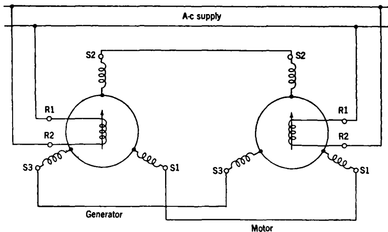
FIG. 10-11.—Synchro generator-motor system.
