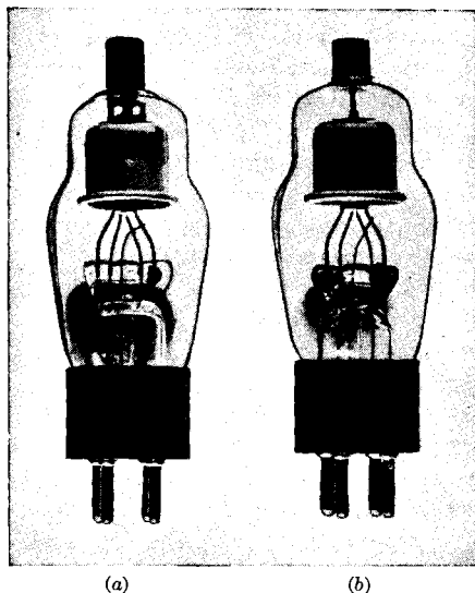
FIG. 14-3.—"Ruggedized" and standard 2X2's. (a) Ruggedized (2B21); (b) standard 2X2.
