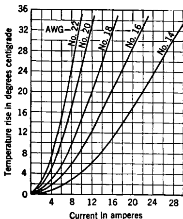
FIG. 1-2.—Temperature rise vs. current.
