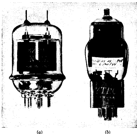
FIG. 14-18.—Small transmitting beam tetrodes. (a) 829B, Ken-Rad; (b) 3D21, Hytron.
