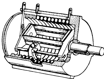
FIG. 8-24.—Helipot construction.
