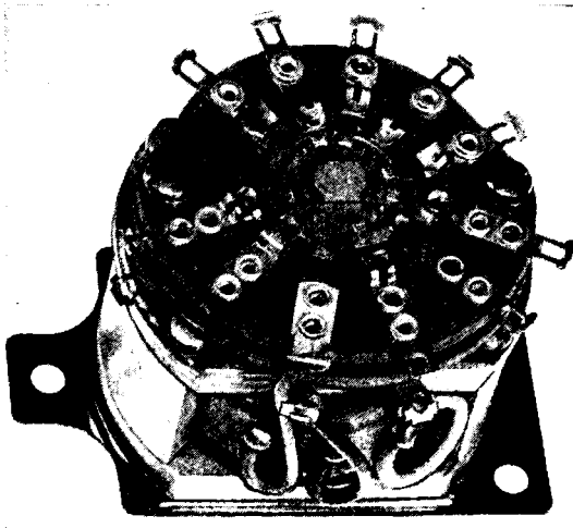
FIG. 13-8.—Price Brothers Company, Type 76-4 relay (No. 97, Table 13-5).
