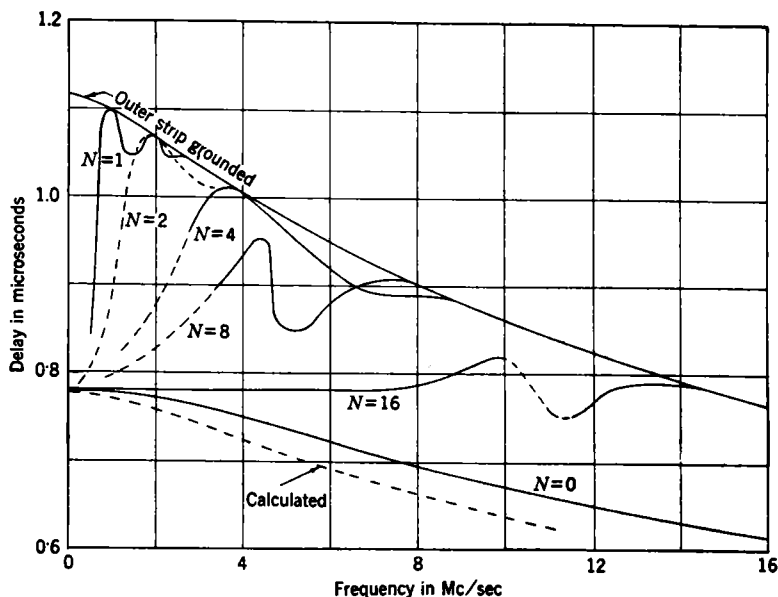
FIG. 6-7.—Effect of subdivision of floating capacitance strip.
