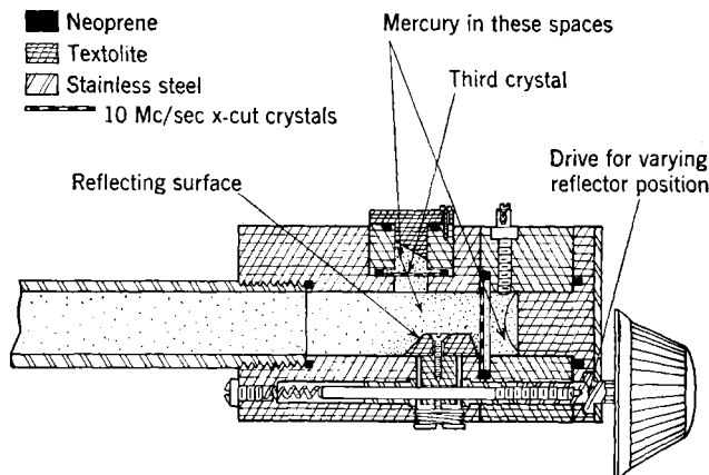
FIG. 7-19.—Variable reflector and third crystal.
