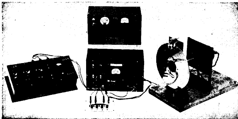
FIG. 8-20.—Point-measurement linearity test assembly.
