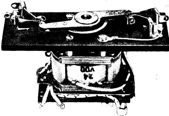
FIG. 13-9.—Price Brothers Company, antenna-transfer relay.
