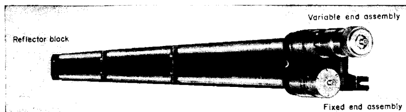
FIG. 7-23.—Line D, assembled.
