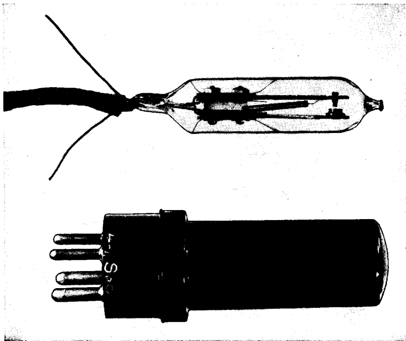
FIG. 13-6.—Thomas A. Edison, Inc., thermal time-delay relay.
