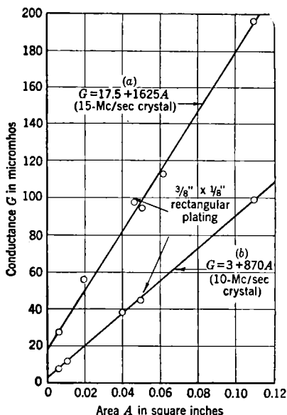
FIG. 5-5.—Conductance of quartz crystal vs. back-plating area. All front platings \frac{1}{8} -in. diameter. All back platings circular except as indicated.
