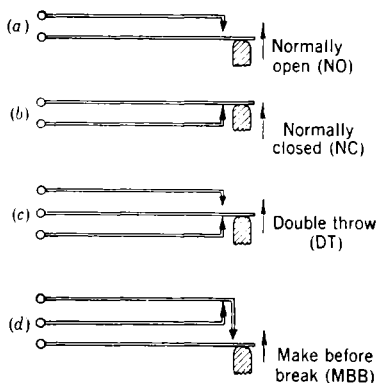
FIG. 13-1.—Basic relay-contact groups.
