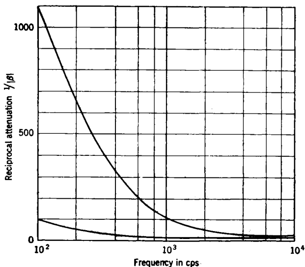
FIG. 9-9.—Attenuation with Western Electric condenser. Upper curve: load resistance 10^6 ohms, shunt capacitance 11 \mu\mu f . Lower curve: load resistance 10^7 ohms, shunt capacitance 1 \mu\mu f .
