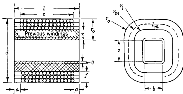
FIG. 4-27.—Dimensions of layer-wound coil. r_m = \frac{r_o + r_i}{2} = \frac{nd_w + (n-1)t_i}{k_b} ; l_m = 2(b + s + \pi r_m) = length of mean turn; f = build of winding; n = number of layers; d_w = OD of wire; t_i = thickness of interlayer insulation (this must be multiplied by a constant to allow for lapping; for \frac{1}{4} turn lapping the constant is about \frac{5}{8} ); k_b = build factor = 0.85 for average construction (see text).
