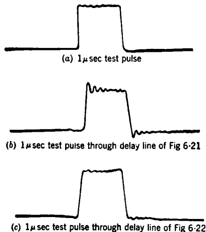
FIG. 6-23.—Waveforms of BTL delay networks. Rise time is 0.2 \mu sec for (b) and 0.1 \mu sec for (c).
