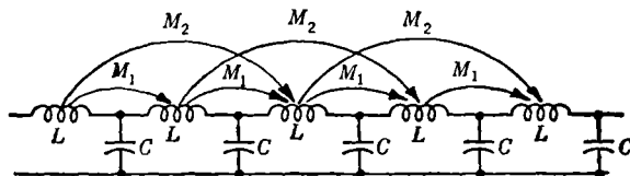
FIG. 6-20.—Mutual inductance between sections of lumped line.
