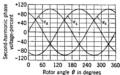
FIG. 10-34.—Second-harmonic phase-voltage distribution in Magnesyne.
