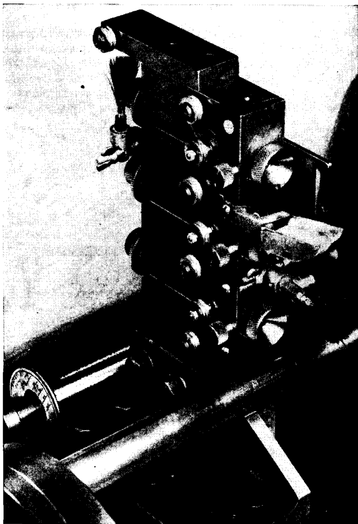
FIG. 8-6.—Carriage of flat-card winding machine.
