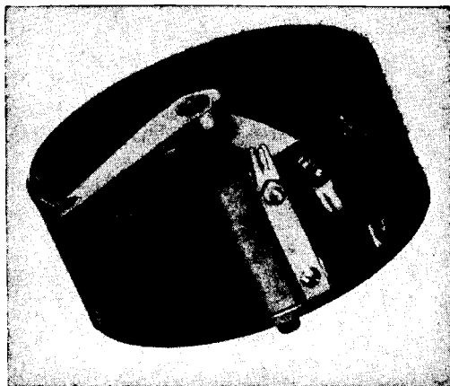
FIG. 8-29.—Muter Type 433A potentiometer.
