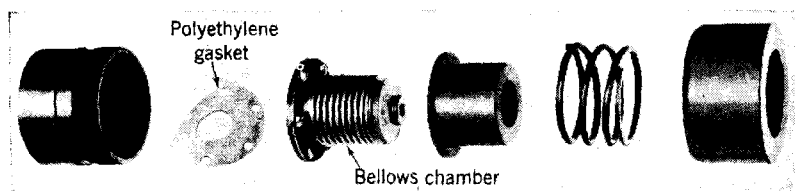
FIG. 7-13.—Pressure bellows for Line E .
