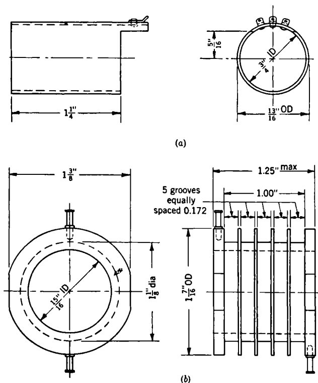
FIG. 4-20.—Primary and secondary coil forms.
