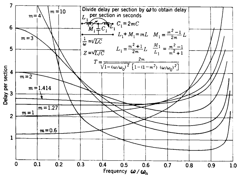
FIG. 6-16.—Delay in m -derived low-pass filter sections.
