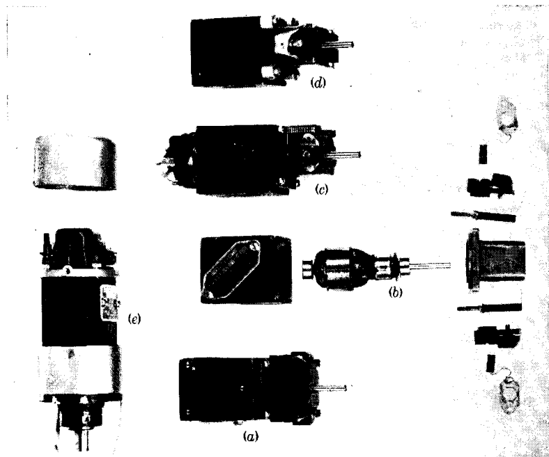
FIG. 11-2.—Deleo midget PM motors. (a) Standard type; (b) standard type, disassembled; (c) standard type with Lee governor; (d) with hinge-type brushes for tachometer use; (e) with integral gear-reduction unit and brush cover.
