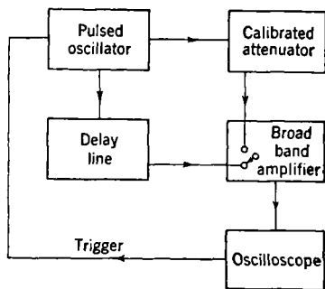
FIG. 7-20.—Block diagram for voltage-loss measurement.
