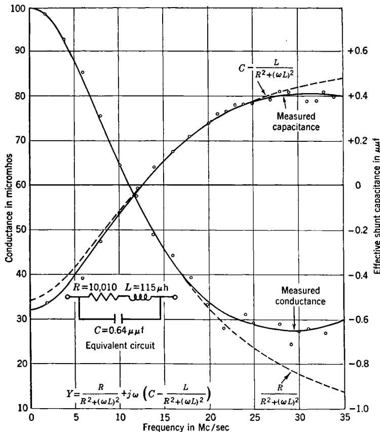
Fig. 3-10.—High-frequency characteristics of IRC type AB resistor.
