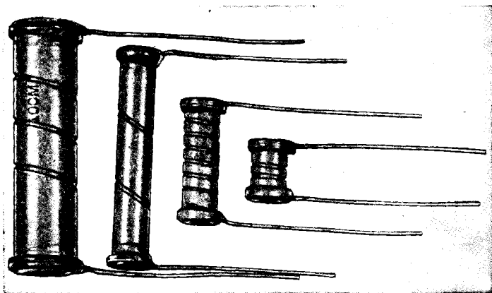
FIG. 3-17.—Continental Carbon Co. precision resistors.
