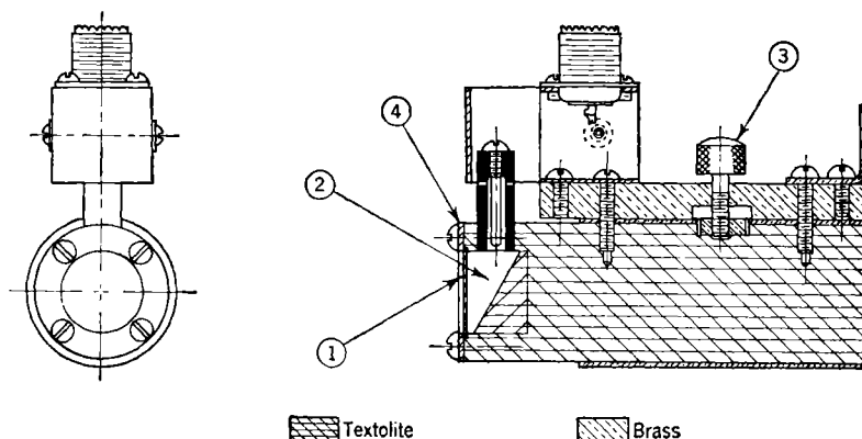
FIG. 7-2.—Crystal assembly for Line A. (1) A 10-Mc/sec crystal, plated on the front side, is lacquered to Textolite piece. (2) This space holds the backing mercury. The main part of the assembly slides inside a tube containing the water. (3) This screw elevates the piece into which it is threaded and so holds the assembly fixed in the tube. Wire leads connect the uhf fitting to the mercury well and to the (grounded) clamp ring (4).
