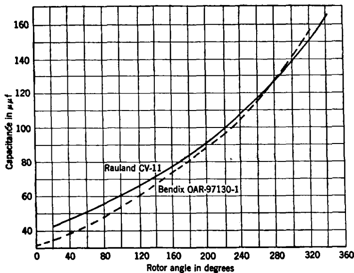
FIG. 9-21.—Capacitance vs. rotor angle.
