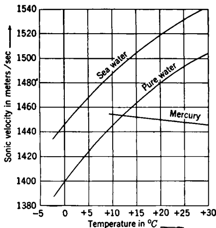
FIG. 7-1.—Sonic velocity as a function of temperature.
