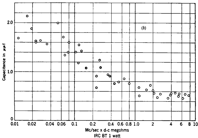
FIG. 2-25.—Total capacitance-frequency characteristics.
