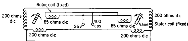
FIG. 10-39.—Telegon system schematic diagram.
