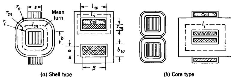
FIG. 4-1.—Iron-core inductor dimensions.
