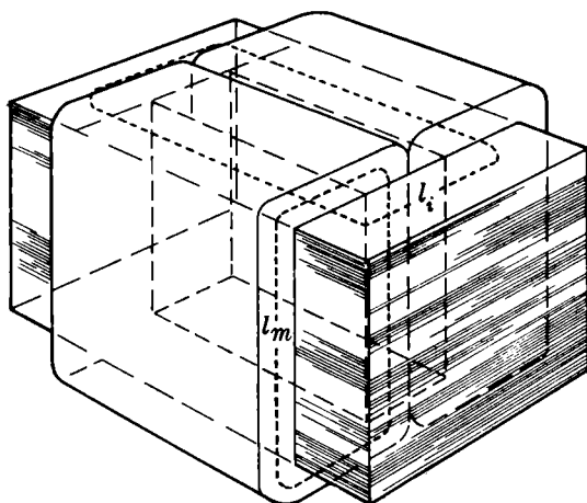
FIG. 4-15.—Core-type transformer with balanced coils.
