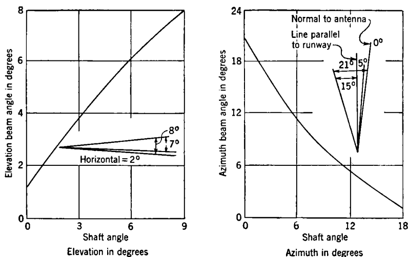
FIG. 9-14.—Beam position vs. shaft angle.
