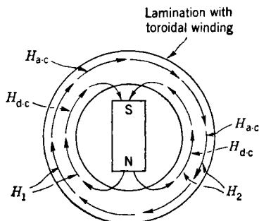
FIG. 10-30.—Magnetomotive forces in Magnesyn core.
