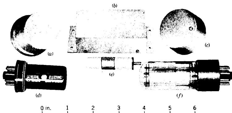
FIG. 5-2.—A collection of crystal types showing external appearances.
