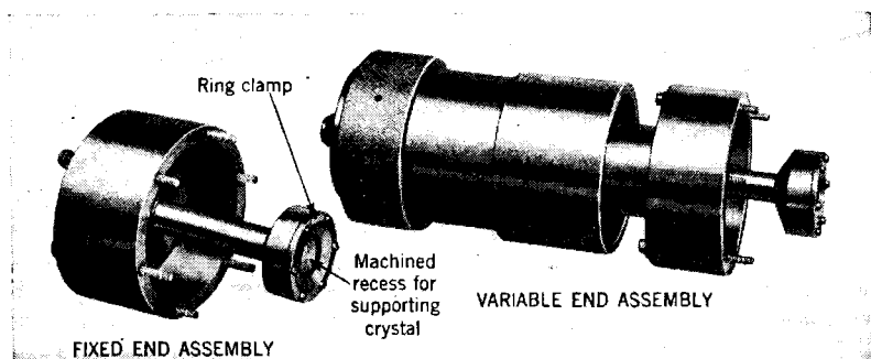
FIG. 7-8.—End assemblies for Line D.
