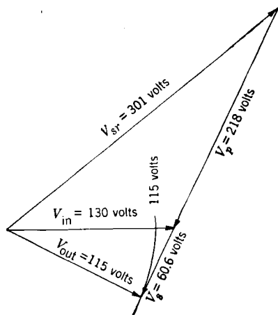
FIG. 12-45.—Vector diagram for maximum input voltage.
