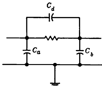
FIG. 2-20.—Equivalent circuit including ground capacitances.
