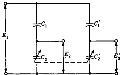
FIG. 9-13.—Push-pull capacitive voltage divider.
