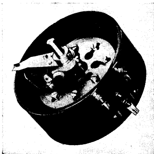
FIG. 8-15.—General Radio Company type 433-AC potentiometer.
