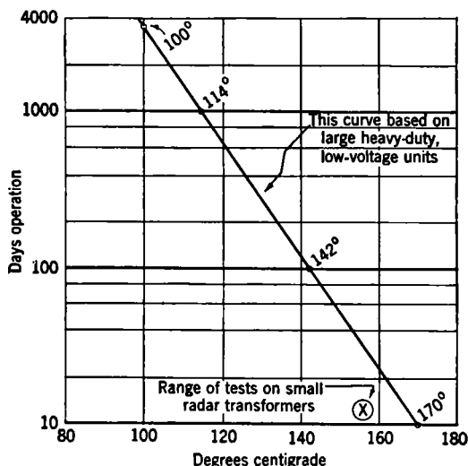
FIG. 4-13.—Transformer life vs. operating temperature.
