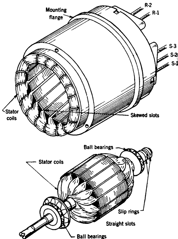
FIG. 10-8.—Synchro control transformer.
