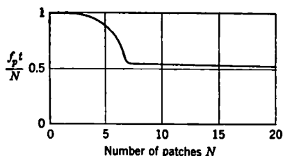
FIG. 6-8.—Wavelength per patch at peak.
