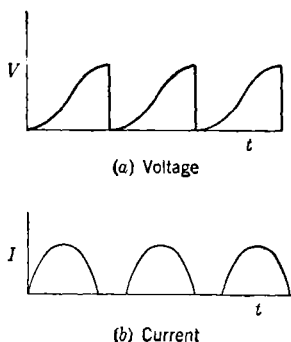
FIG. 4-10.—Voltage and current waveforms in resonant-charging choke.
