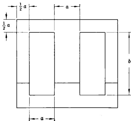
FIG. 4-23. Radiation Laboratory standard nickel-iron laminations.
