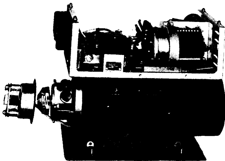
Fig. 12-17.—Wincharger Corporation aircraft motor alternator with Holtzer-Cabot speed control.
