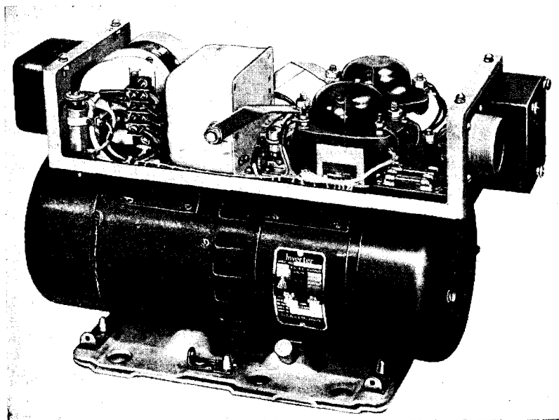
FIG. 12-12.—Leland Electric Company aircraft motor alternator with regulator.
