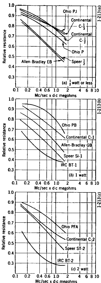
Fig. 2-23.—Resistance-frequency characteristics (3).
