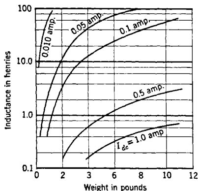
FIG. 4-9.—Filter-choke inductance as a function of weight.
