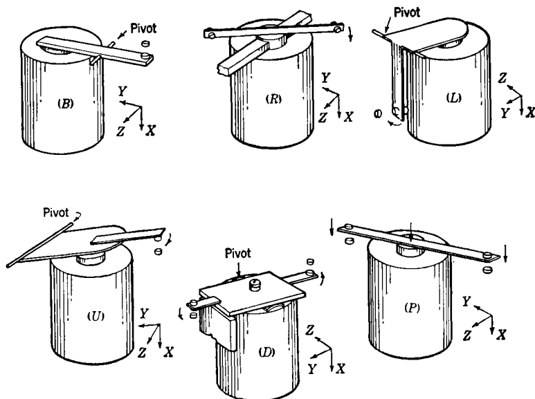
FIG. 13-30.—Relay armature and contact structures.
