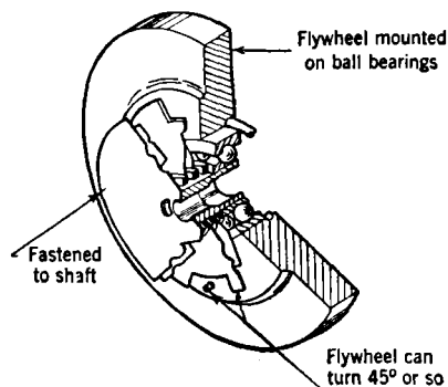
FIG. 10-6.—Synchro-motor damping flywheel.
