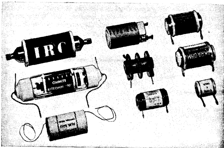
Fig. 3-13.—Typical accurate wire-wound resistors.
