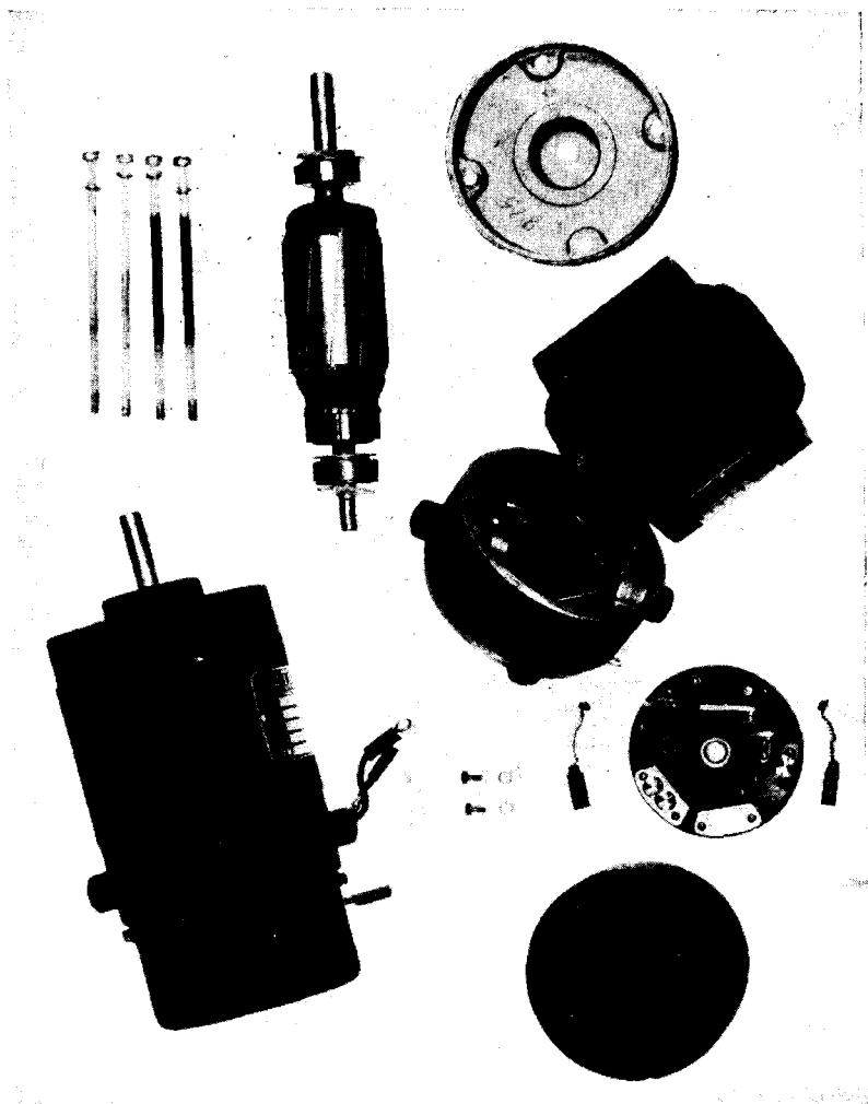
FIG. 11-23.—Diehl constant-speed d-c series motor: 27-volt input, \frac{1}{80} hp, 6000 rpm, with Lee centrifugal governor.
