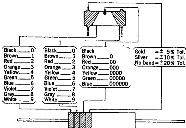
FIG. 2-2.—Standard color code for fixed composition resistors.
