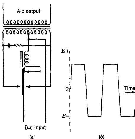
FIG. 12-24.—Shunt vibrator circuit with buffer condenser.
