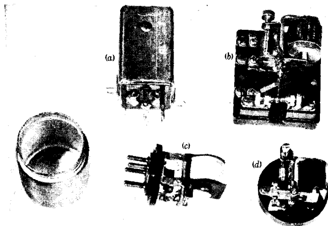
FIG. 13-26.—Typical sensitive relays. (a) Sigma 4RHPL; (b) Allied BD-330; (c) General Electric CR2791C104C23 with cover removed; (d) Allied G.
