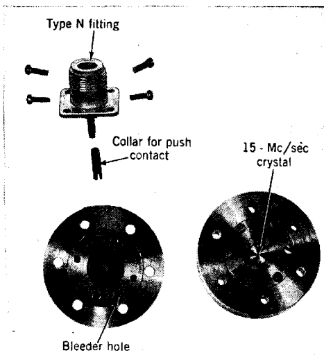
FIG. 7-11.—End assembly, Line E.
