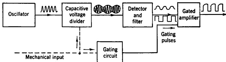
FIG. 9-11.—Generation of sweep-voltage wave.
