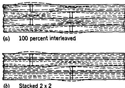
FIG. 4-16.—Flux paths at lamination lap joints.
