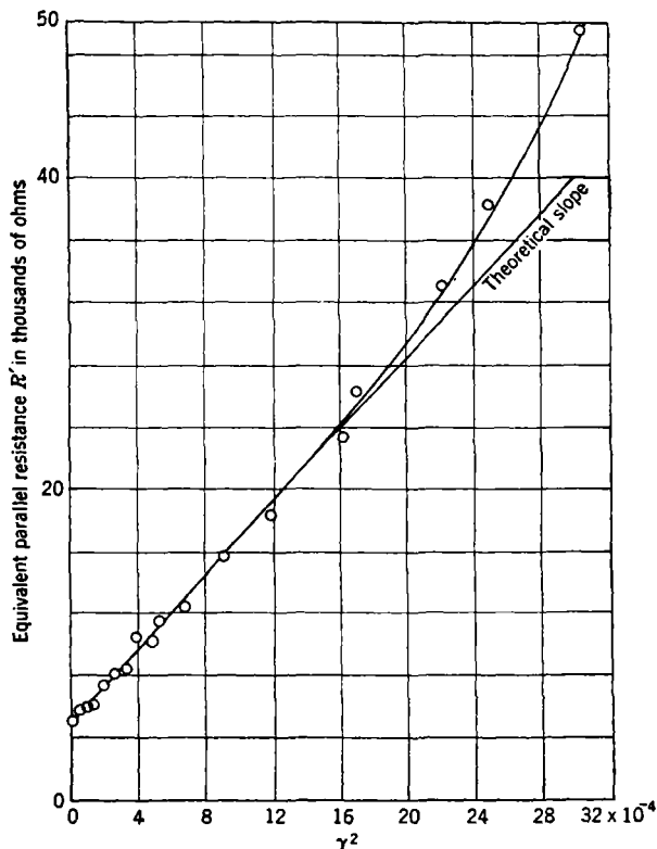
FIG. 5-6.—Validity of equivalent circuit of Fig. 5-4. Equivalent parallel resistance R' [from Eqs. (1) and (2)] is plotted as a function of \gamma^2 . Theoretical slope is R_s Q_s , where R_s = 4.7k and Q_s = 16 .
