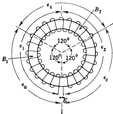
FIG. 10-33.—A-c flux and voltage distribution in Magnesyne.
