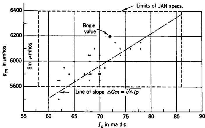
Fig. 14-16.—Variations in characteristics of 6L6GA tubes.
