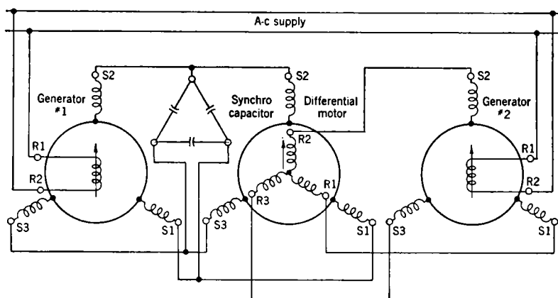
FIG. 10-13.—Differential synchro system.
