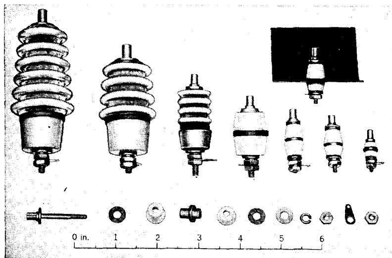
FIG. 4-28.—Rubber-sealed bushings.
