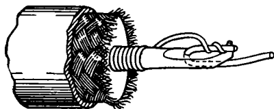
FIG. 1-12.—Method of terminating inner conductor.
