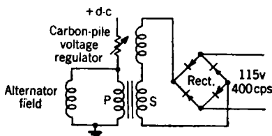
FIG. 12-31.—Schematic diagram of stabilizing transformer in voltage-regulator circuit of 400-cps aircraft inverter.
