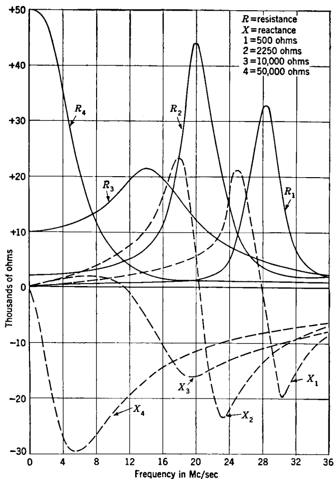
Fig. 3-11.—High-frequency characteristics of wire-wound resistors.
