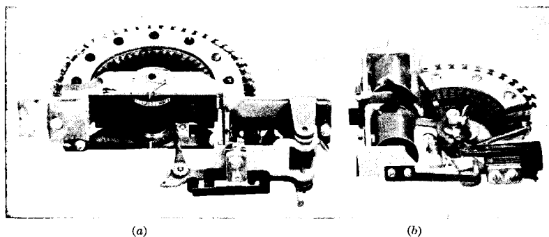
FIG. 13-19.—Stepping switches. (a) Western Electric D87856-F10; (b) Automatic Electric 204E.
