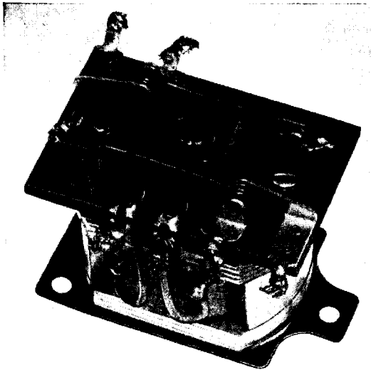
FIG. 13-7.—Price Brothers Company, Type 311 relay (No. 99, Table 13-5).
