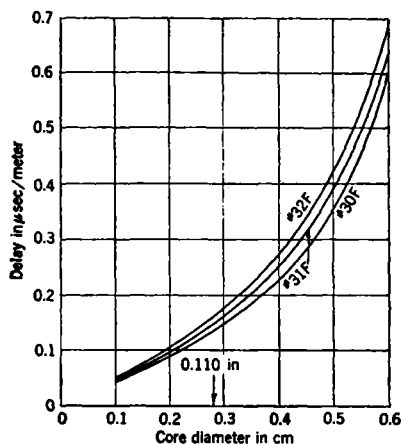
FIG. 1-10.—Delay vs. core diameter.
