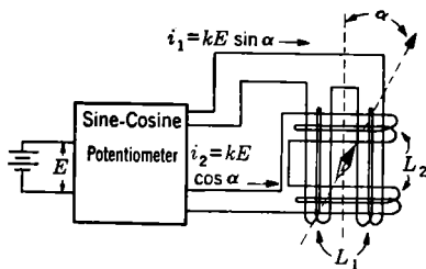
FIG. 10-42.—Principle of d-c Selsyn operation.
