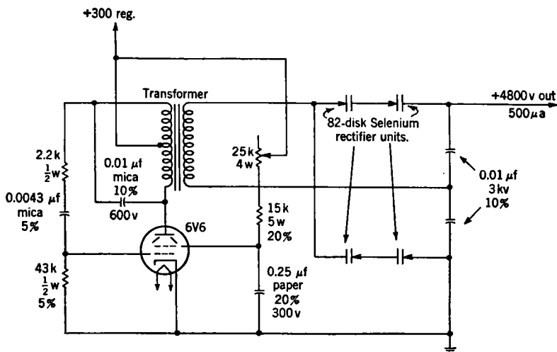
FIG. 4-18.—A-f oscillator power supply.
