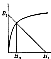
FIG. 4-3. — Graphical determination of operating point.
