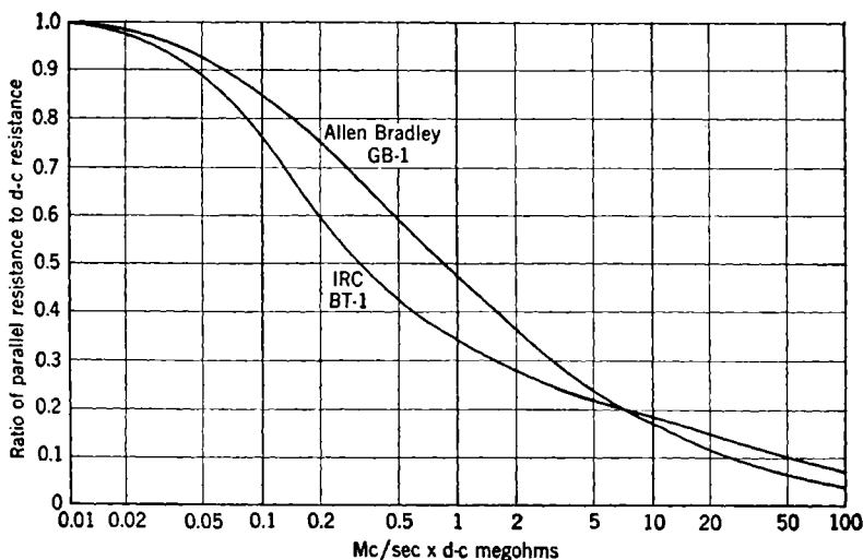
FIG. 2-22.—Resistance-frequency characteristics (2).
