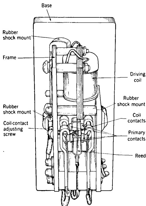
FIG. 12-20.—Typical heavy-duty vibrator.
