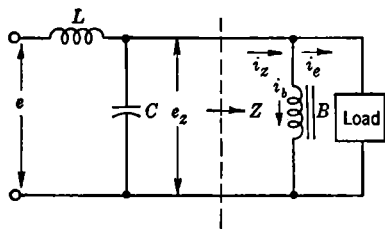
Fig. 12-36.—Simplified equivalent circuit of saturable-transformer voltage regulator.
