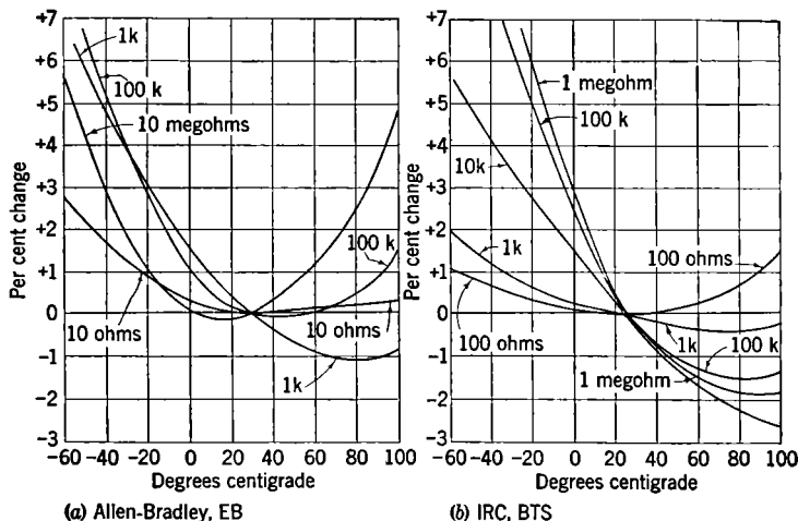
FIG. 2-12.—Resistance-temperature characteristics (2).
