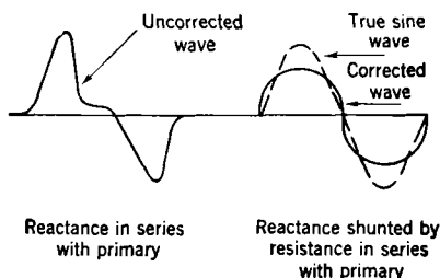
FIG. 12-46.—Waveform corrections in voltage stabilizer.
