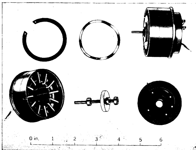
FIG. 10-29.—Mechanical construction of a Magnesyn.
