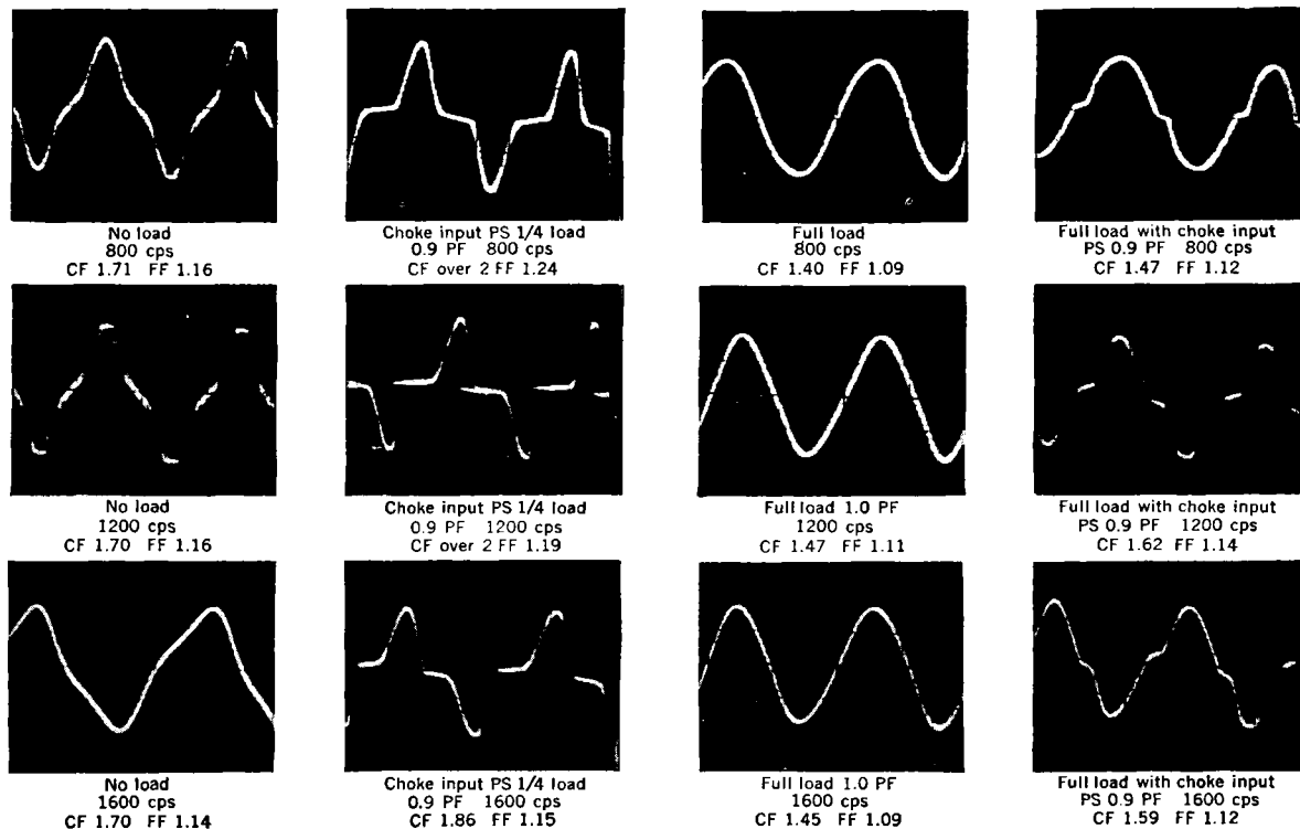
FIG. 12-8.—Voltage waveshape of Eclipse NEA-6 generators.
