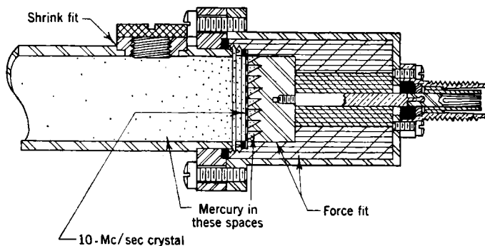
FIG. 7-6.—End assembly with sawtooth backing.
