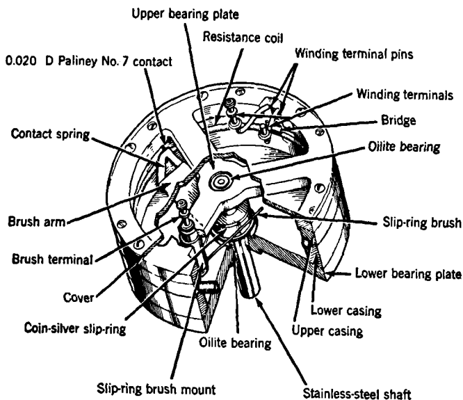
FIG. 8-25.—RL-270 potentiometer construction.
