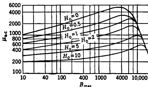
FIG. 4-4.—Incremental permeability curves for Allegheny Audio Transformer "A" sheet steel.
