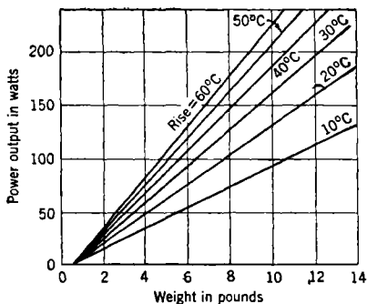
FIG. 4-11.—Power output vs. weight.
