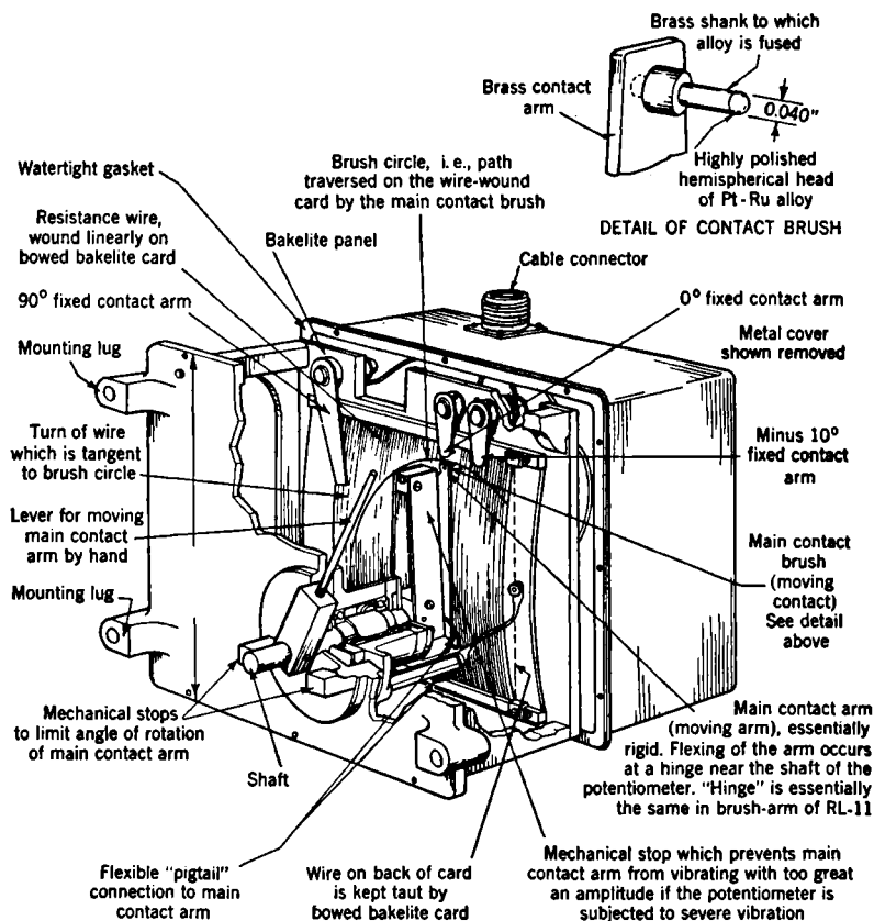
Fig. 8-33.—RL-204 potentiometer construction.
