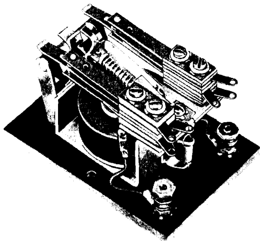
FIG. 13-2.—Advance Electric Company type 904A indexing relay.
