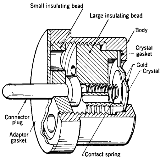
FIG. 5-3.—Supersonic crystal cartridge.
