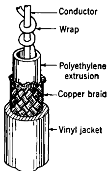
FIG. 1-5.—Section of RG-62/U cable.
