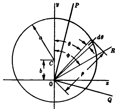
FIG. 9-7.—Geometry of circular rotor.
