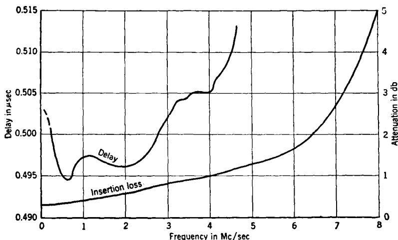
FIG. 6-21 (a and b).—BTL type D-168435 delay line.
