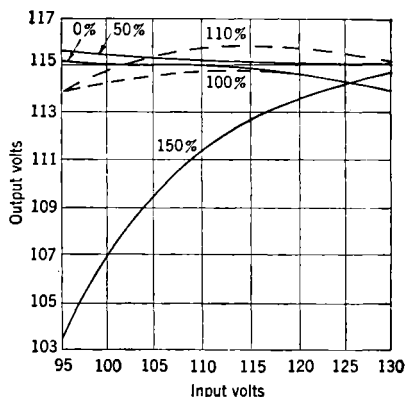
FIG. 12-39.—Regulation curves with resistive load; figures on curves give per cent of full load.
