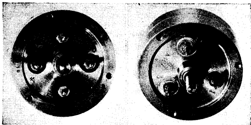
FIG. 9-4a.—Western Electric condenser. FIG. 9-4b.—Nilsen condenser.
