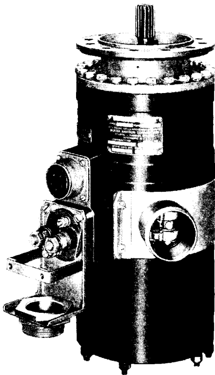
FIG. 12-3. Eclipse NEA-7 dual-voltage generator.
