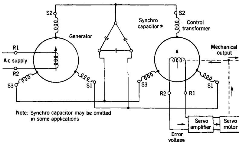
FIG. 10-12.—Synchro generator-control transformer-servo system.
