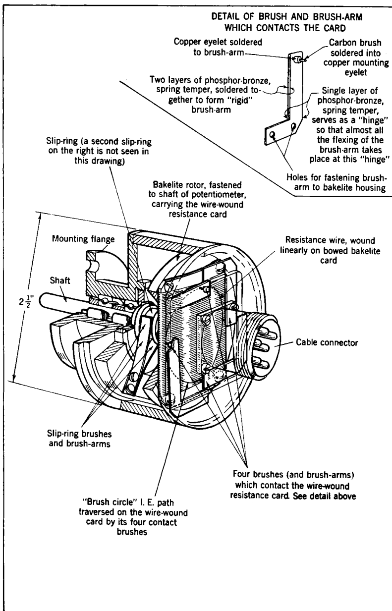
FIG. 8-16.—Construction of potentiometer, type RL-11.
