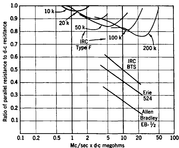
FIG. 2-24.—Resistance-frequency characteristics (4).
