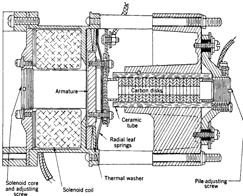
FIG. 12-28.—Carbon-pile voltage regulator (cross section).
