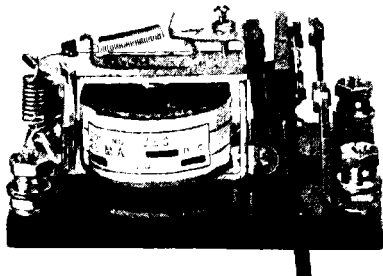
FIG. 13-16.—Leach Relay Company Type 1042-P manual-reset overload relay.
