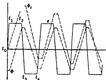
FIG. 12-26.—Voltage and flux in vibrator transformer.
