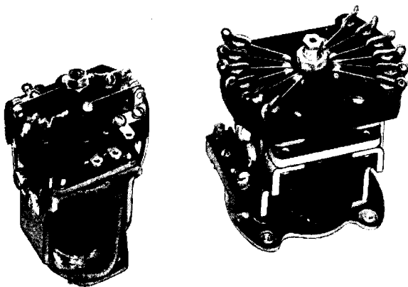
FIG. 13-12.—Allied Control Company experimental DPDT and 4PDT rotary relays.
