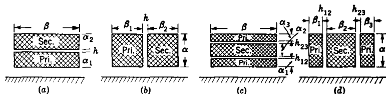
FIG. 4-2.—Coil dimensions.
