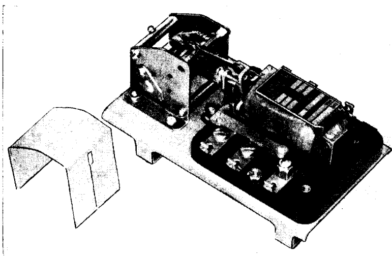
FIG. 13-20.—Escapement-type lag relay, Wheelock RX-9038-2.
