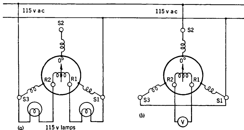
FIG. 10-23.—Zeroing a Navy control transformer. (a) Adjust for minimum brightness. (b) Adjust for zero voltage. The symbol V represents a low-range a-c voltmeter or 2000-ohm headset.
