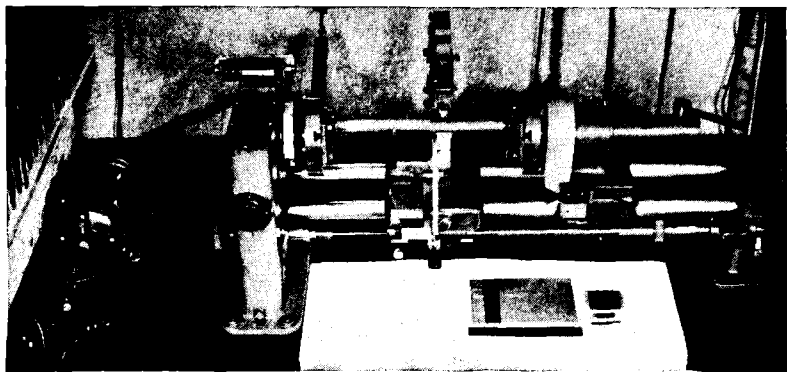
Fig. 8-5.—Flat-card winding machine.
