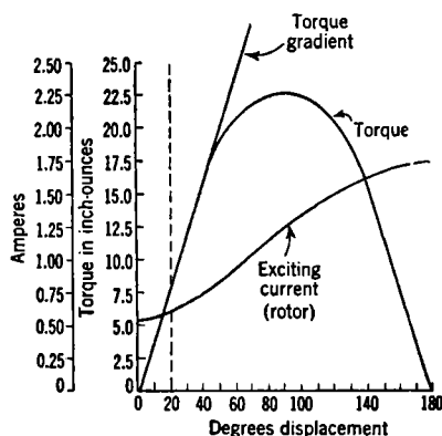
FIG. 10-15.—Typical synchro torque-displacement curve.
