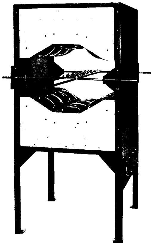
FIG. 4-34.—Infrared soldering oven.
