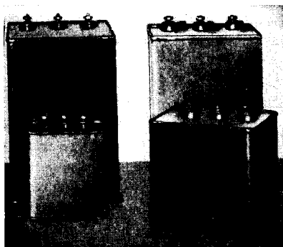
FIG. 10-14a.—Synchro capacitors.
