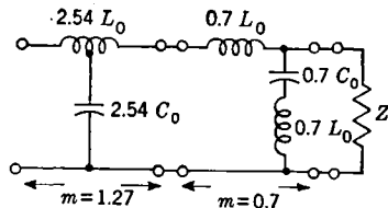
FIG. 6-18.—Termination of lumped-parameter line.
