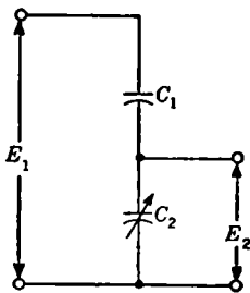
FIG. 9-12.—Simple capacitive voltage divider.
